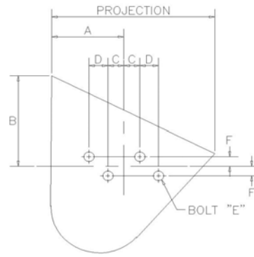
G6 ATTACHMENT
