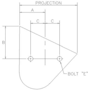
G1 ATTACHMENT
